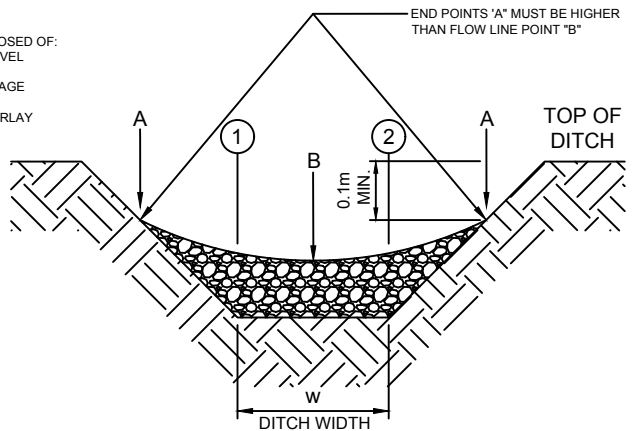
CROSS SECTION
